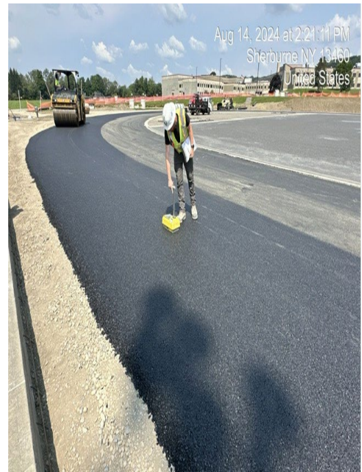
ATL Onsite for Paving Testing
